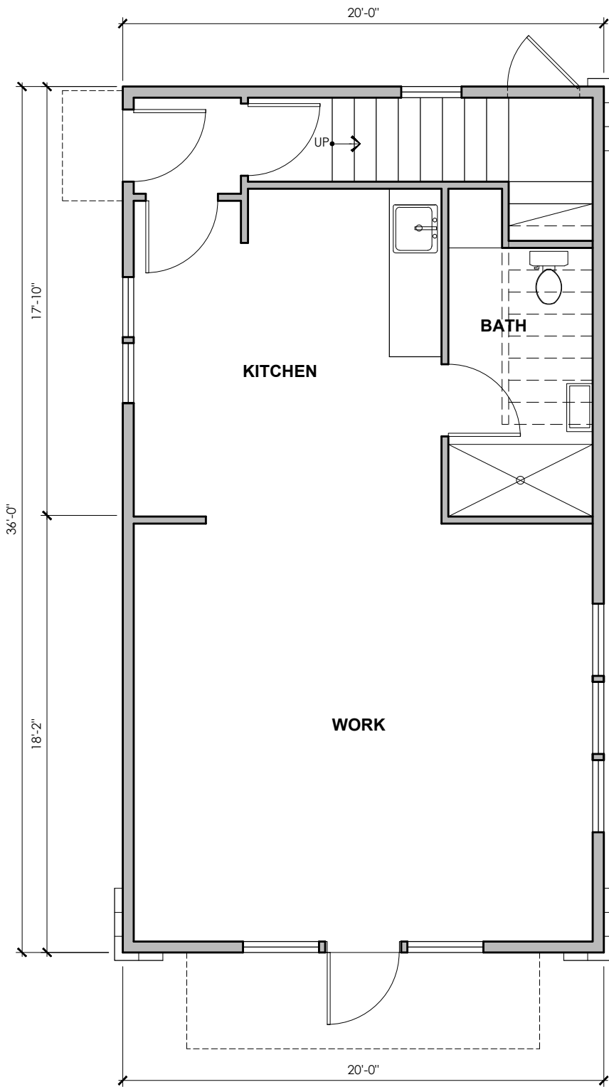
1st FLOOR PLAN - TYP ALL BLDGS AT 304
